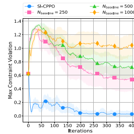
Fig. 10. (Ship Route Planning) Maximum constraint violation of SI-CPPO and baselines versus the number of iterations. The solid line is the maximum constraint violation averaged over 20 random seeds. And we also provide the according error bars.
